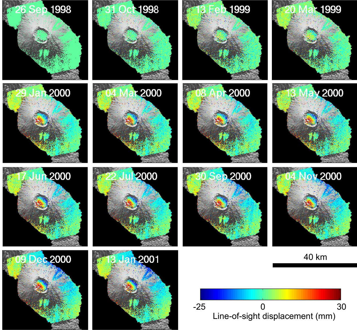
Figure 8. Ascending orbit PS interferograms for Alcedo, plotted on SRTM topography displayed in shaded relief. The data are unwrapped, and spatially correlated error estimates have been subtracted. Displacements are given relative to PS pixels in the southeast and 26 September 1998.
