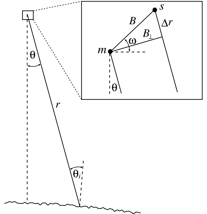
Figure 3. Imaging geometry for satellite radar interferometry. The sensor is moving into the plane of the paper, its position at the time of the “master” acquisition marked by m , and at the time of the “slave” acquisition by s . B is the baseline distance between the sensor positions at the two times, with B_{\perp} being the perpendicular component of B , r is the range from the sensor to the Earth’s surface, \omega is the angle between the baseline vector and the horizontal, \theta is the look angle and \theta_i is the angle of incidence at the Earth’s surface.
