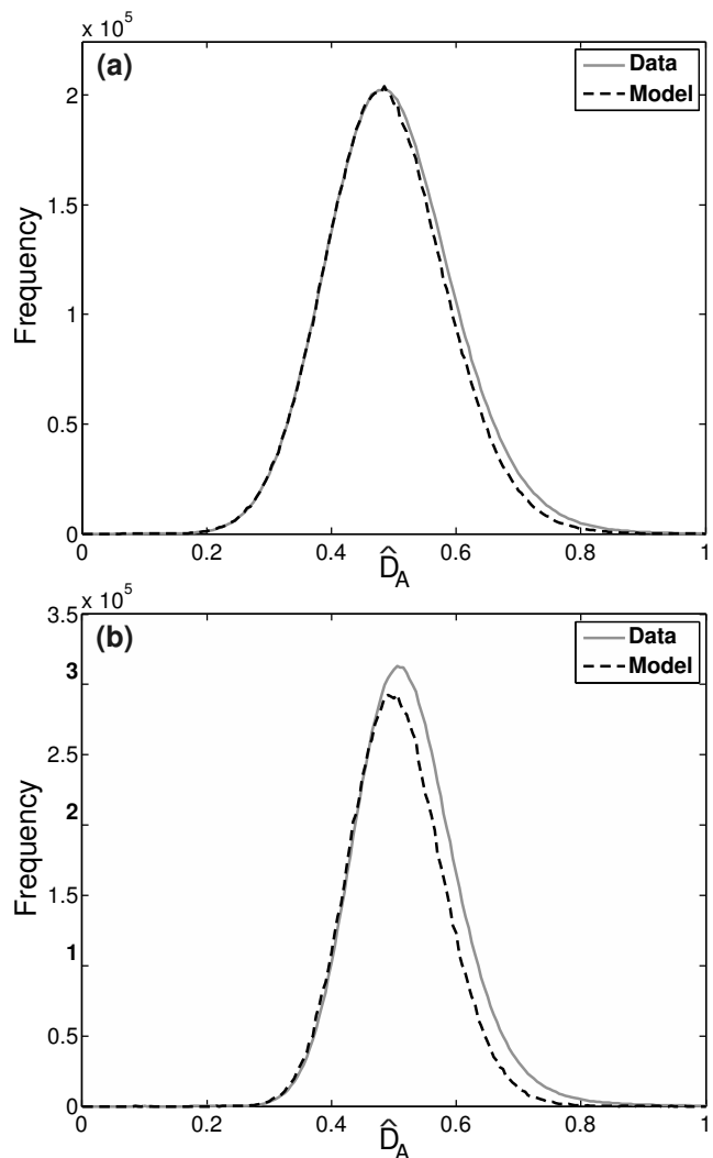
Figure 19. Distribution of amplitude dispersion for (a) 15 images acquired over Volcán Alcedo and (b) 24 images acquired over Mount St. Helens. Also plotted are the distributions predicted from the best-fitting model SNR distributions.
