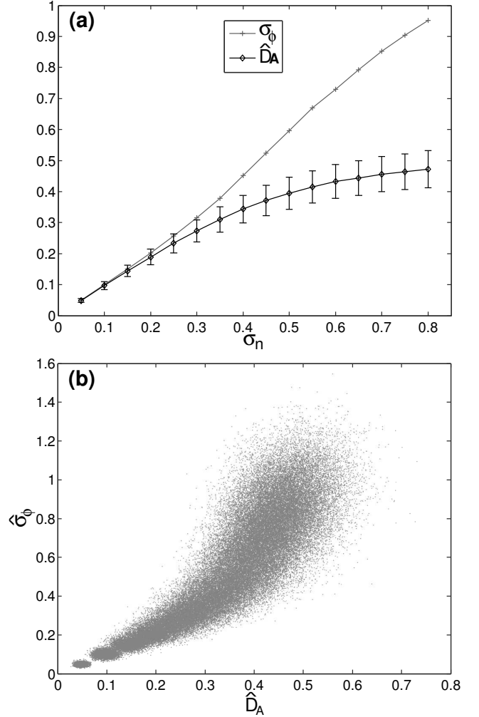
Figure 16. Amplitude dispersion numerical simulation results. The signal model is z_i = g + n_i ( i = 1, \dots, 34 ). The value of g is fixed to 1 while the standard deviation, \sigma_n , of both the real and imaginary components of the noise, n_i , is incremented from 0.05 to 0.8. For each value of \sigma_n , we calculate 5000 estimates of \hat{D}_A . In (a) the mean values of \hat{D}_A are plotted for each value of \sigma_n , as in Ferretti et al. [2001], with error bars representing one standard deviation. Also plotted are corresponding values of phase standard deviation, \sigma_\phi . In (b), the same data are plotted in a scatter plot of the estimated phase standard deviation, \hat{\sigma}_\phi , vs. \hat{D}_A for all values of \sigma_n .
