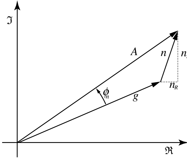
Figure 21. Model for pixel amplitude, A . The signal is assumed to have constant amplitude, g . The real and imaginary components of the noise, n_R and n_I , are characterized by the same Gaussian distribution.
