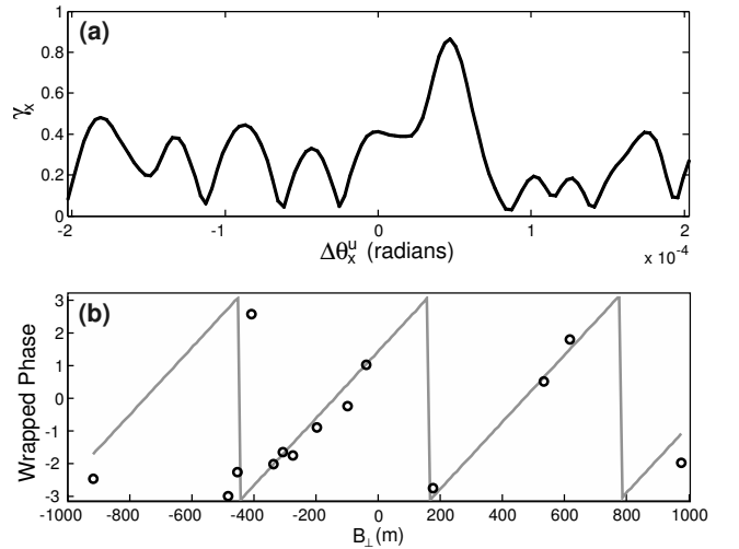
Figure 4. An example parameter space search for look angle error, \Delta\theta_x^u , for a PS pixel in the Alcedo descending orbit data set (see Section 6). (a) shows the goodness of fit for trial values of \Delta\theta_x^u and (b) shows a comparison between the data (circles) and phase values predicted by the value of \Delta\theta_x^u with maximum \gamma_x (grey line).
