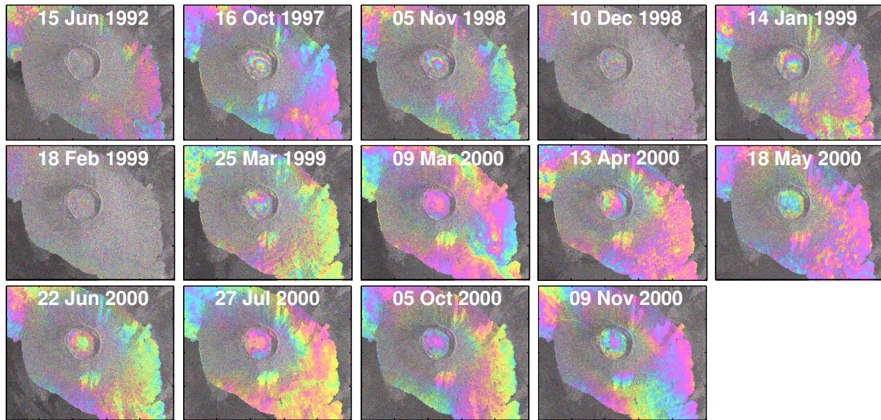
Figure 5. Wrapped interferograms in radar coordinates formed from descending orbit data acquired over Alcedo, with 4 looks taken in range and 20 in azimuth. The “master” acquisition date is 03 February 2000. Each color fringe represents 2.8 cm of displacement in the LOS and the intensity reflects interferogram amplitude.
