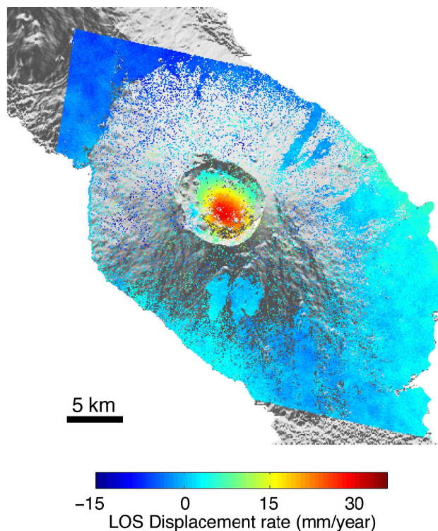
Figure 11. Mean LOS velocities on Alcedo between October 1997 and November 2000 from descending orbit data. The velocities are relative to the mean velocity of PS pixels on the coasts.
