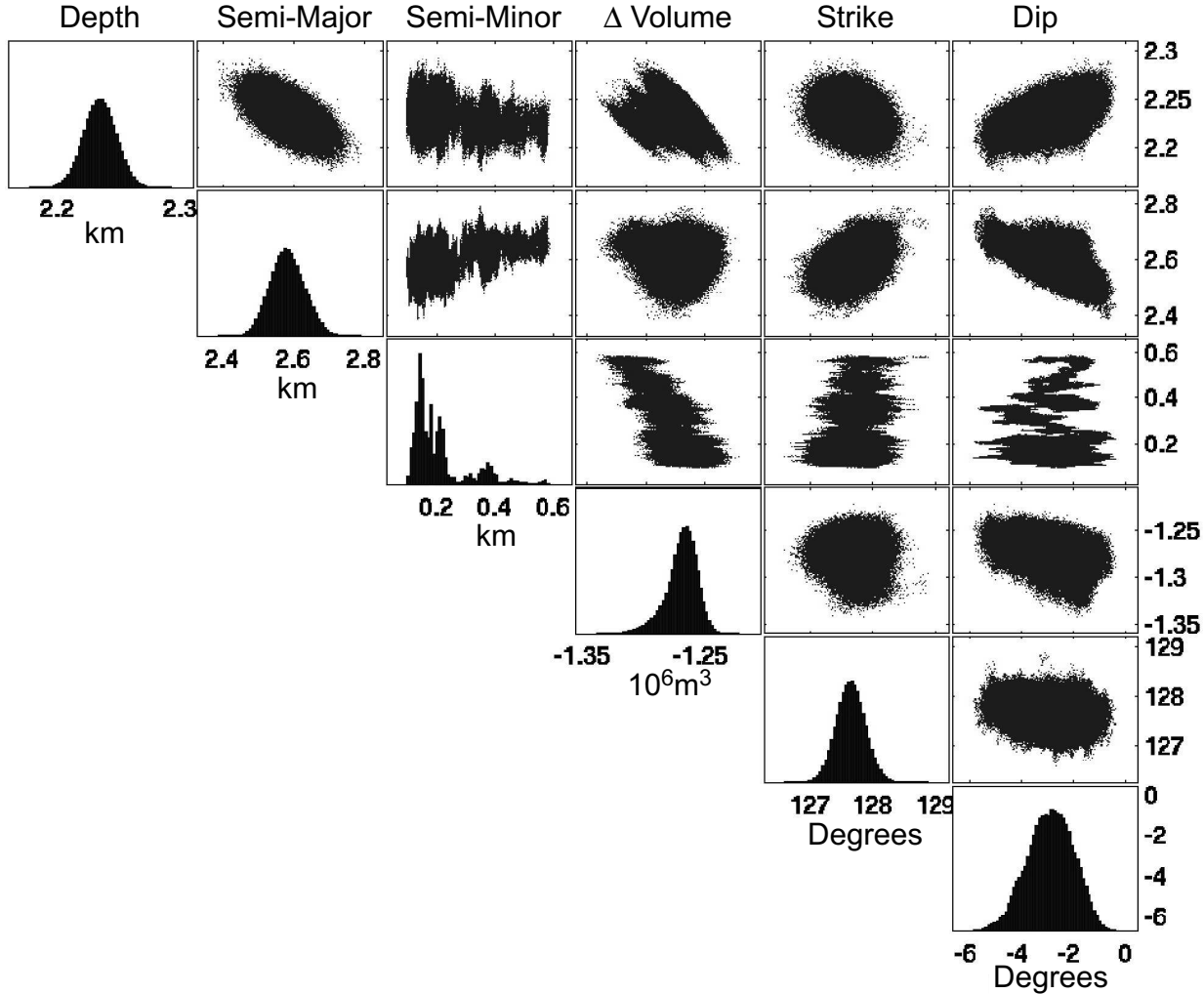
Figure 15. Marginal posterior probability distributions for ellipsoidal source model parameters. The histograms show the distributions for individual parameters and the scatter plots show distributions for each pair of parameters.
