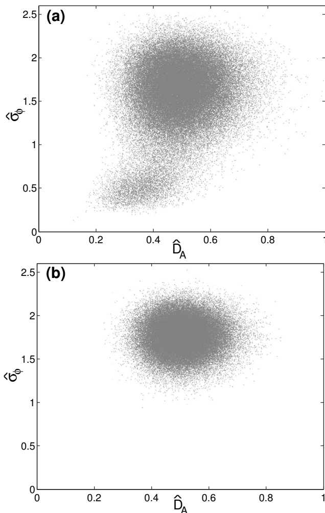
Figure 20. Scatter plots of simulated phase standard deviation vs. amplitude dispersion for model distributions of SNR for (a) Volcán Alcedo and (b) Mount St. Helens.
