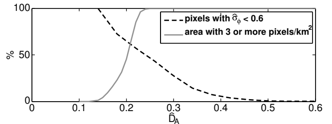
Figure 18. Percentage of high phase stability pixels ( \hat{\sigma}_\phi \leq 0.6 ) for different threshold values of \hat{D}_A , given our model distributions of noise standard deviation for data acquired over Volcán Alcedo.
