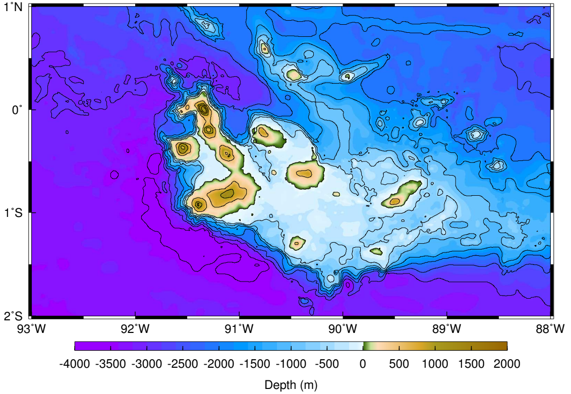
Figure 17. Bathymetry of the Galápagos region, from data compiled by William Chadwick, Oregon State University. The contour interval is 500 m.
