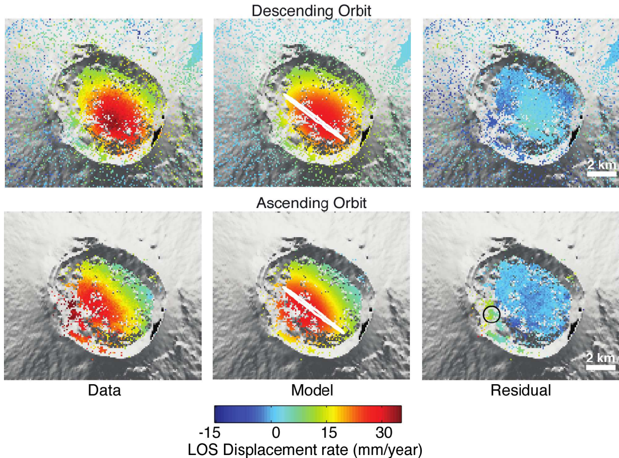
Figure 12. Maximum likelihood model for PS pixels on the caldera floor. The LOS velocities of PS pixels are shown, together with the velocities predicted by the model, and the residual between the two. The ellipse overlaying the predicted velocities is the surface projection of the maximum likelihood ellipsoid contracting source. The circle overlaying the ascending data marks the location of the PS pixels used for landslide analysis in Section 6.2.
