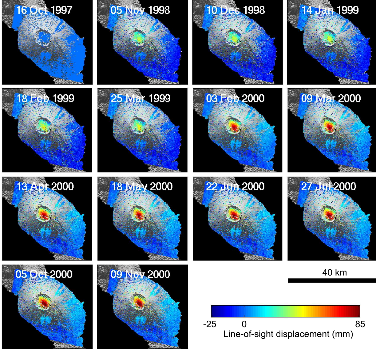
Figure 7. Descending orbit PS interferograms for Alcedo, plotted on SRTM topography displayed in shaded relief. The data are unwrapped, and spatially correlated error estimates have been subtracted. Displacements are given relative to PS pixels in the southeast and 16 October 1997.
