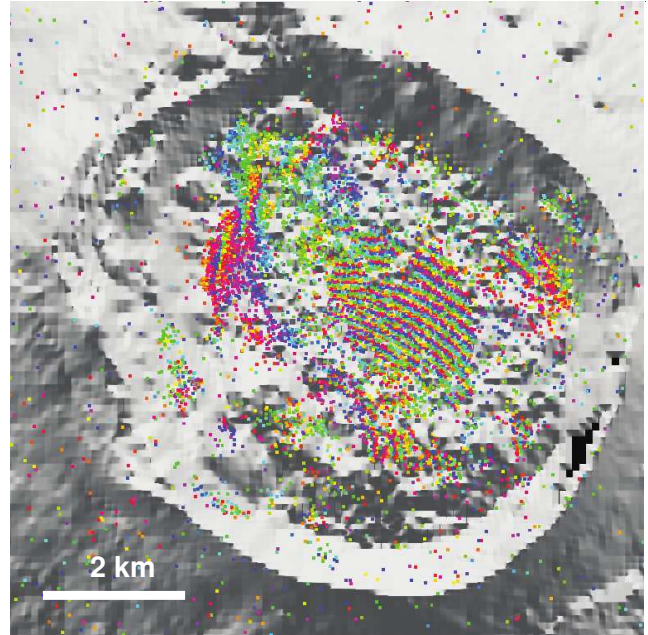
Figure 9. Wrapped PS interferogram for Alcedo caldera covering the interval 15 June 1992 to 05 November 1998. The background image is SRTM topography in shaded relief. Each color fringe represents 2.8 cm of displacement in the LOS and the southern end of the fringes is moving toward the satellite with respect to the northern end.
