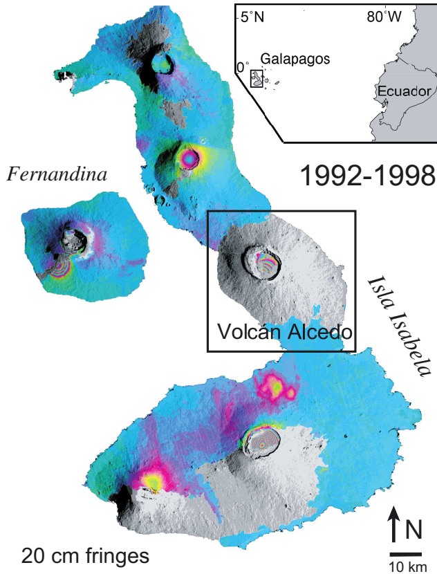
Figure 1. Location of Volcán Alcedo on Isla Isabela, Galápagos. The background image from Amelung et al. [2000], shows line-of-sight displacement between 1992 and 1998.
