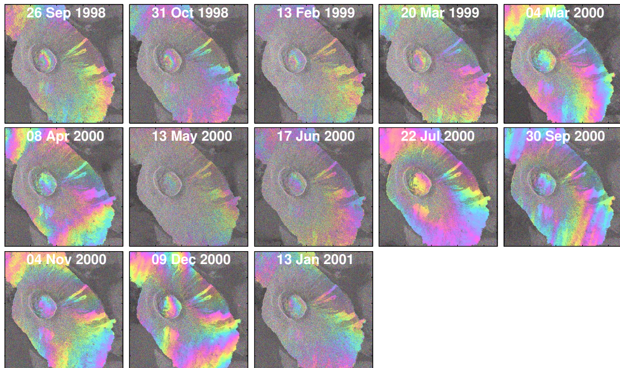
Figure 6. Wrapped interferograms in radar coordinates formed from ascending orbit data acquired over Alcedo, with 4 looks taken in range and 20 in azimuth. The “master” acquisition date is 29 January 2000. Each color fringe represents 2.8 cm of displacement in the LOS and the intensity reflects interferogram amplitude.
