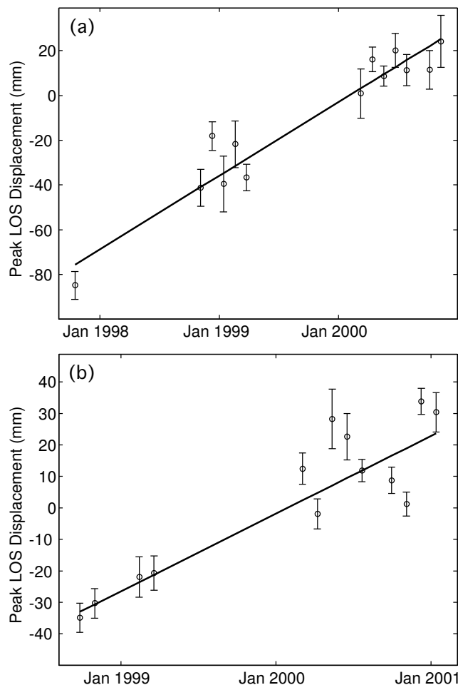
Figure 10. Maximum LOS displacements on Alcedo. For each PS interferogram the mean LOS displacement of the region of maximum displacement is plotted. For the descending case the displacements are relative to PS pixels near the coasts and for the ascending case the displacements are relative to PS pixels on the east side of the caldera. Error bars represent one sample standard deviation. To avoid any bias caused by temporal smoothing, the displacements are calculated before spatially correlated terms are subtracted, which causes extra scatter. Also plotted is the best-fitting constant LOS velocity in each case.
