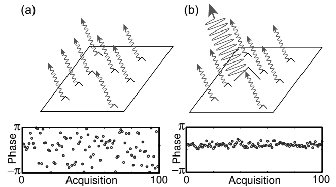
Figure 2. Phase simulations for (a) a distributed scatterer pixel and (b) a persistent scatterer pixel. The cartoons above represent the scatterers contributing to the phase of one pixel in an image and the plots below show simulations of the phase for 100 iterations, with the smaller scatterers moving randomly between each iteration. The brighter scatterer in (b) is three times brighter than the sum of the smaller scatterers.
